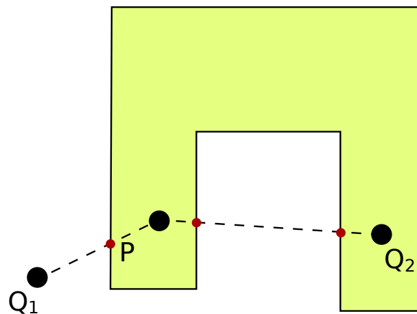
Figure 169: Counting how many times we hit the perimeter gives us the result
